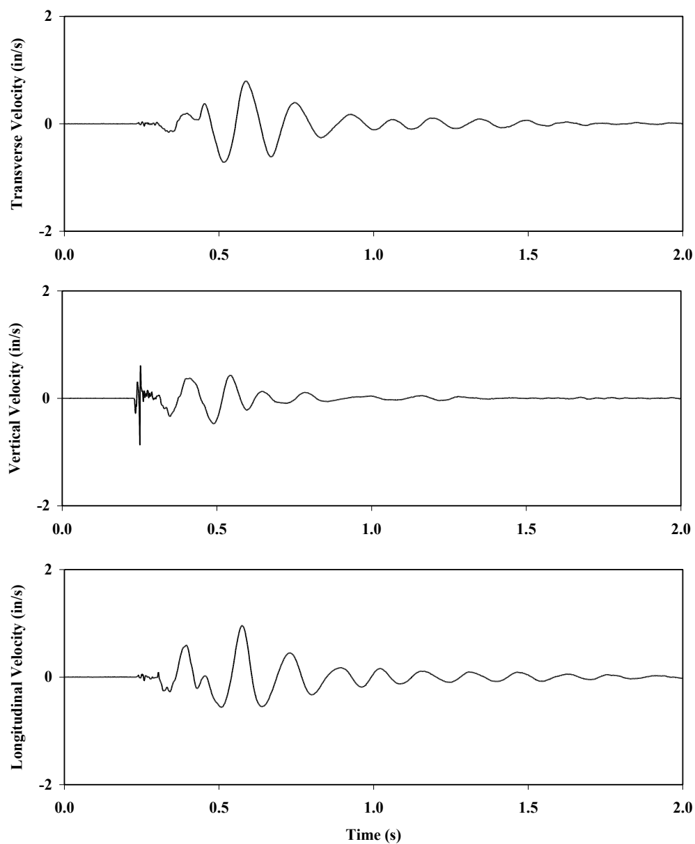
Streambed vibrations recorded during shot D11
