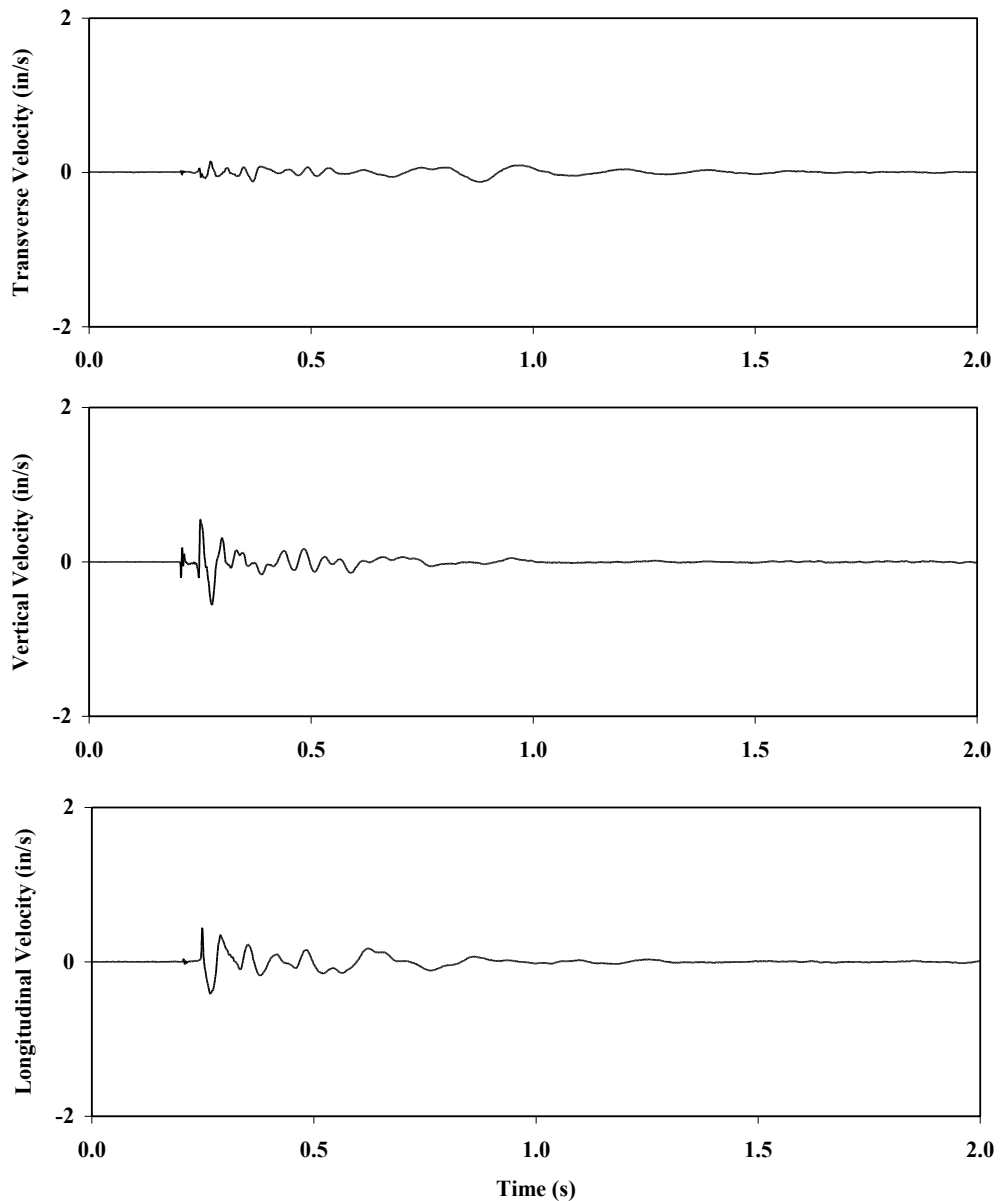
Streambed vibrations recorded during shot D2-2
