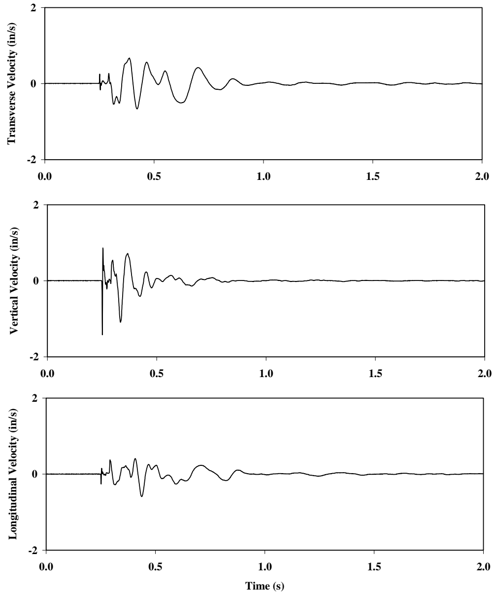
Streambed vibrations recorded during shot D2-1
