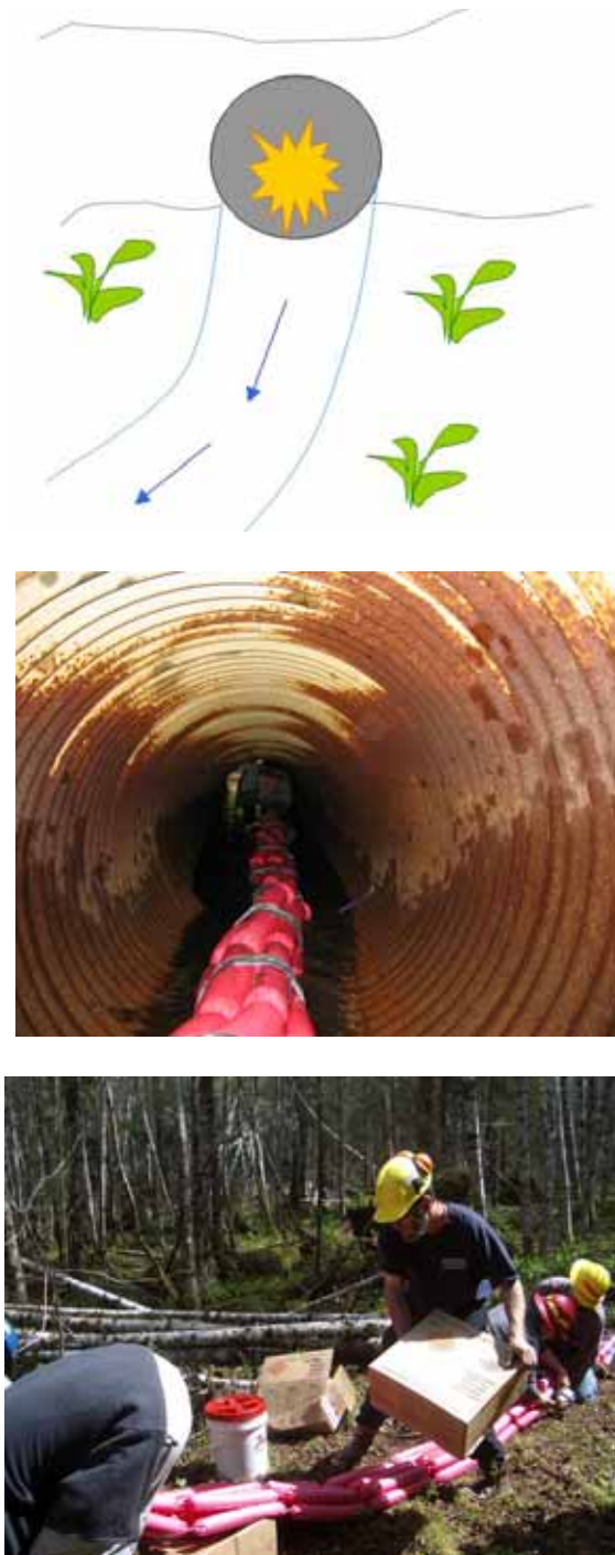
Figure A1.5 Metal culvert explosive design. Top: typical explosive placement for removing a metal culvert. Middle: lengths of emulsion are bound together and pulled through the culvert. Bottom: assembling lengths of emulsion prior to placement.
